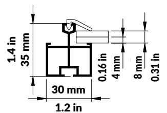
Roof and wall profile
