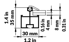
Wall profile for all 3 depths and roof profile for 1.58 m (5.2 ft) depth
