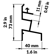
Wall profile for all 3 depths and roof profile for 1.58 m (5.2 ft) depth
