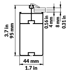
Roof profile for 2.32 m (7.6 ft) and 3.06 m (10 ft) depth
