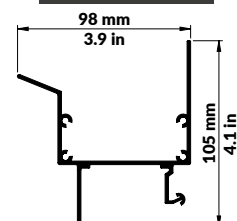
Rain gutter profile
