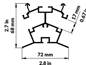
Ridge profile
