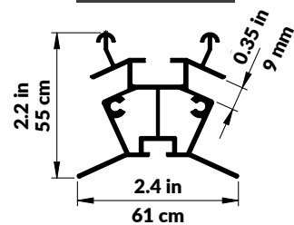
Ridge profile
