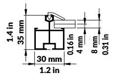
Wall profile for all 3 depths and roof profile for 1.58 m (5.2 ft) depth
