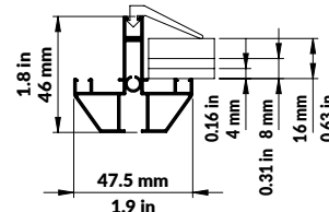
Roof and wall profile
