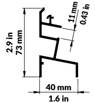
Wall profile for all 3 depths and roof profile for 1.58 m (5.2 ft) depth
